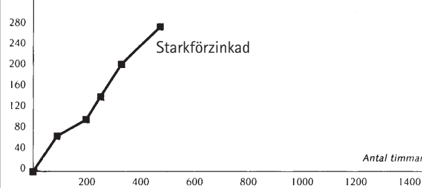
SALT SPRAY TEST (DIN SS50021-ASTM B117/85)
